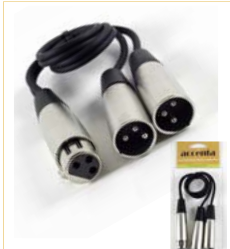
ACC-557 18" XLR Female to Dual XLR Male Cable. 200/CTN
